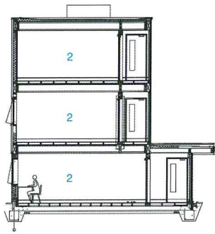
Cross section
